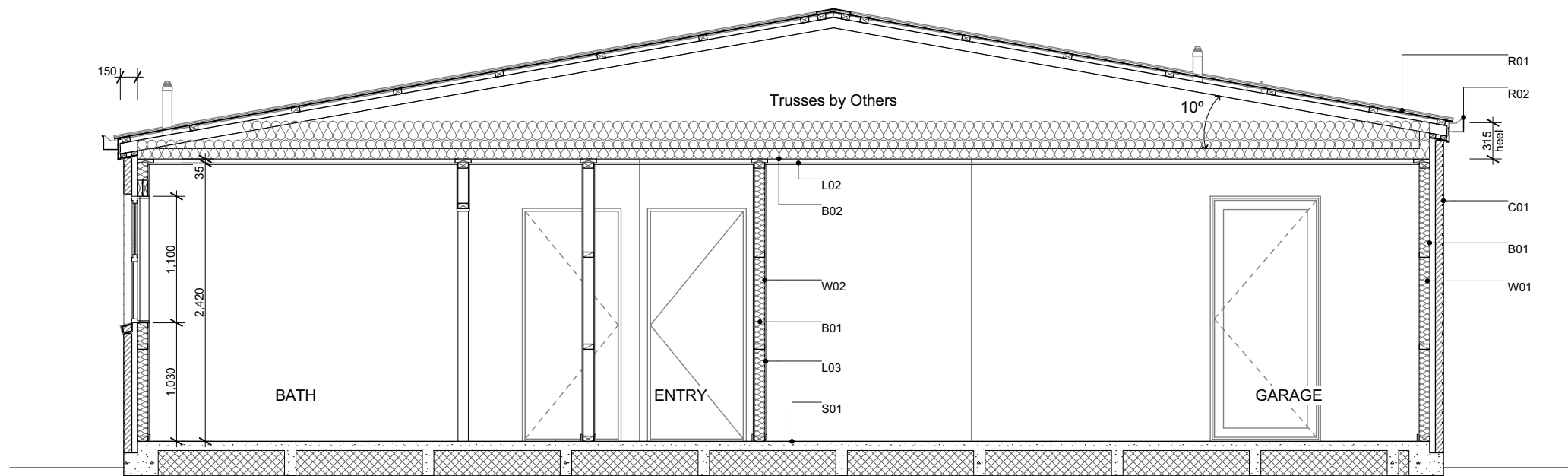
A Section A-A Scale 1:50
