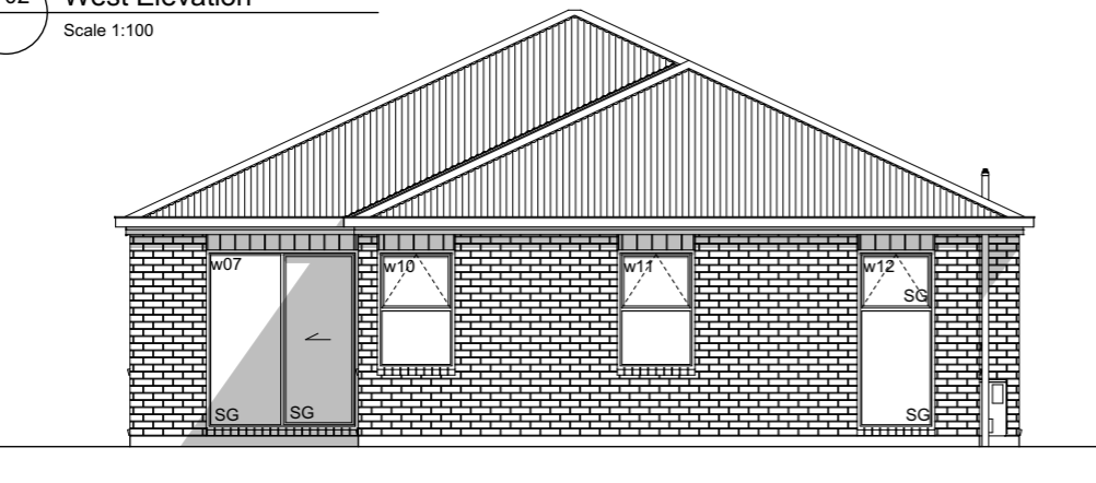
E-03 South Elevation Scale 1:100
