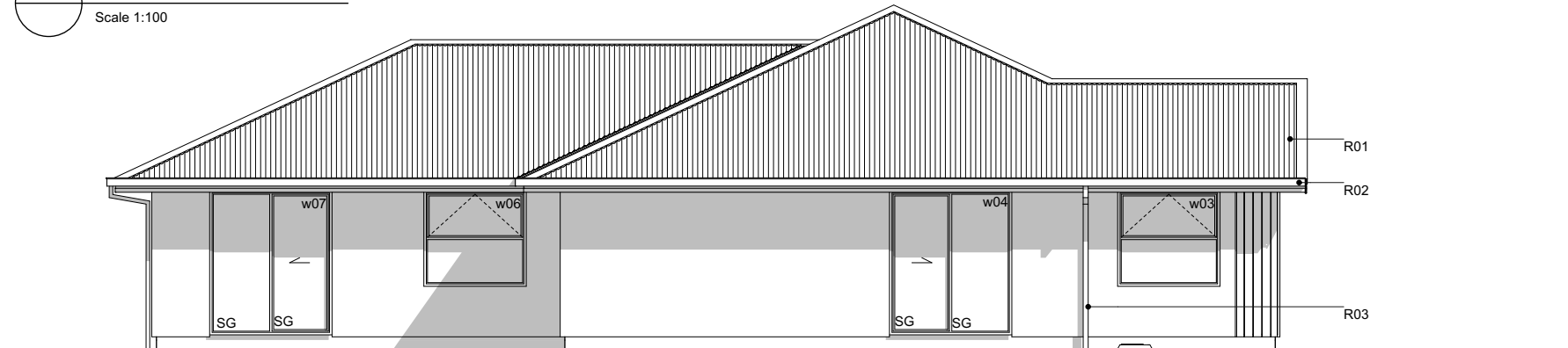
E-02 NorthEast Elevation Scale 1:100
