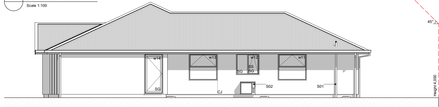
E-04 SouthWest Elevation Scale 1:100
