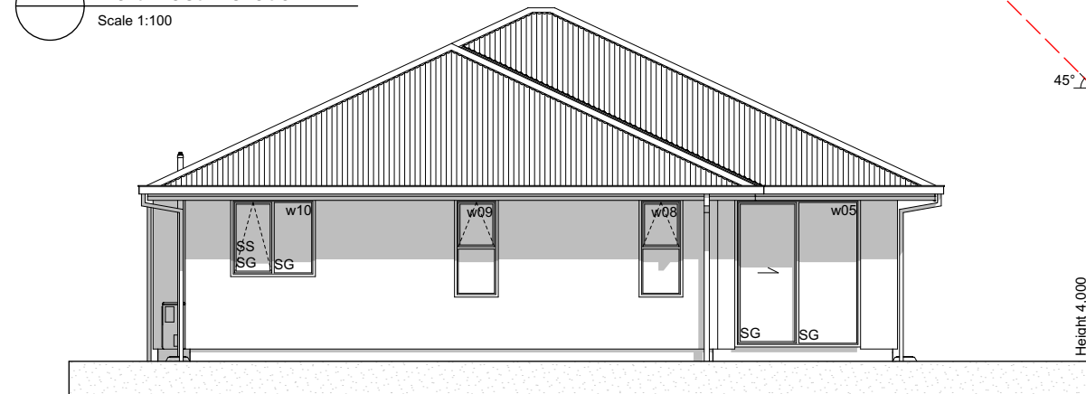
E-03 SouthEast Elevation Scale 1:100
