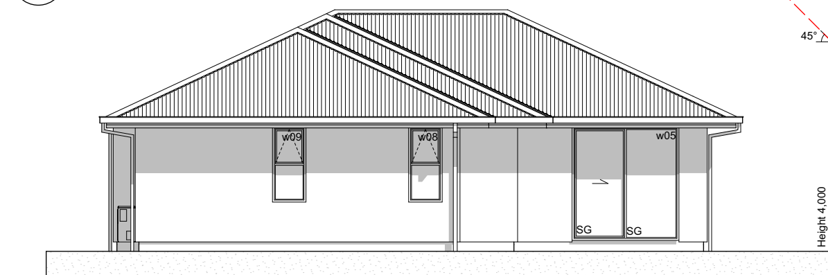
E-03 SouthEast Elevation Scale 1:100
