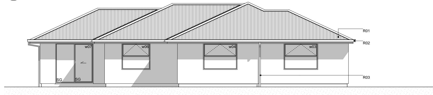
E-02 NorthEast Elevation Scale 1:100
