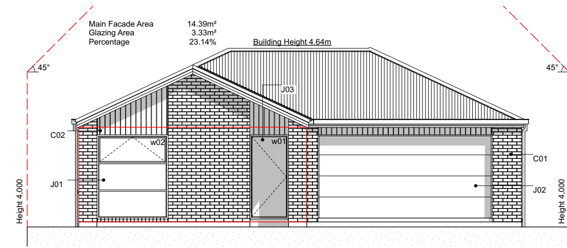
E-01 SouthEast Elevation Scale 1:100
