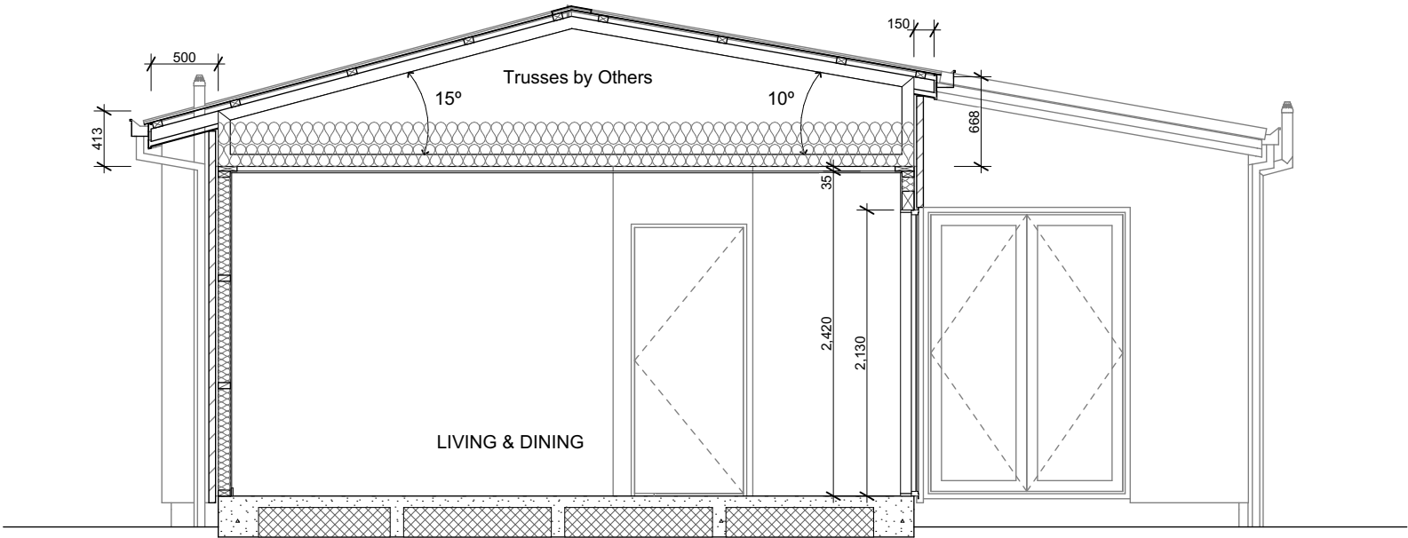
C Section C-C Scale 1:50
