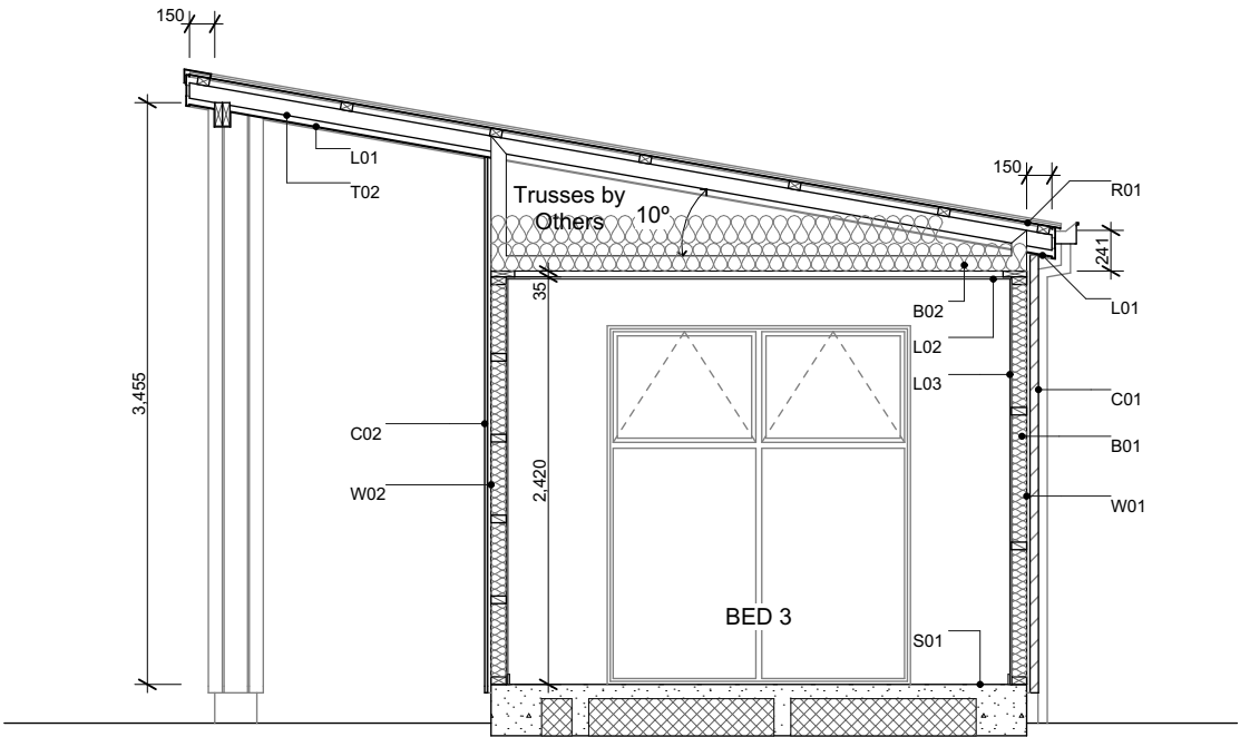
A Section A-A Scale 1:50
