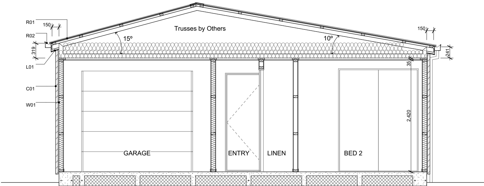
B Section B-B Scale 1:50
