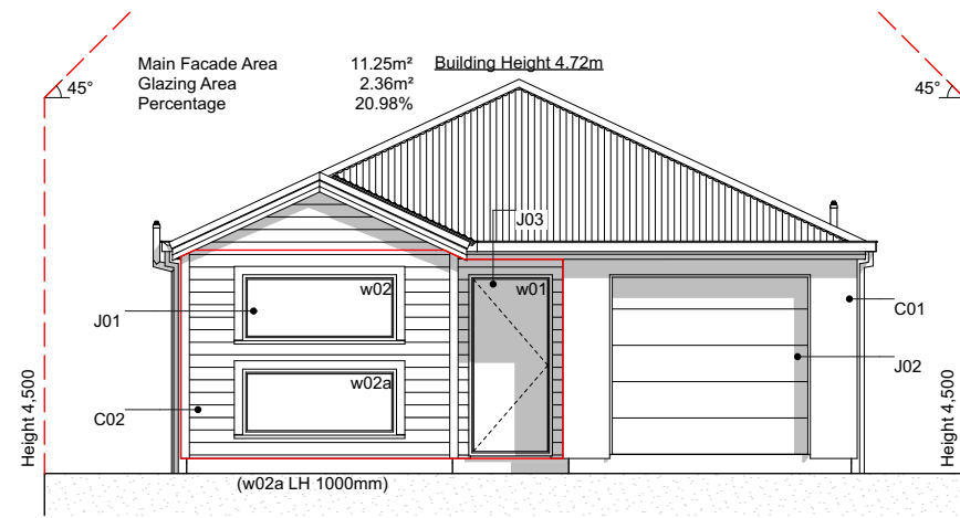
E-01 SouthEast Elevation Scale 1:100
