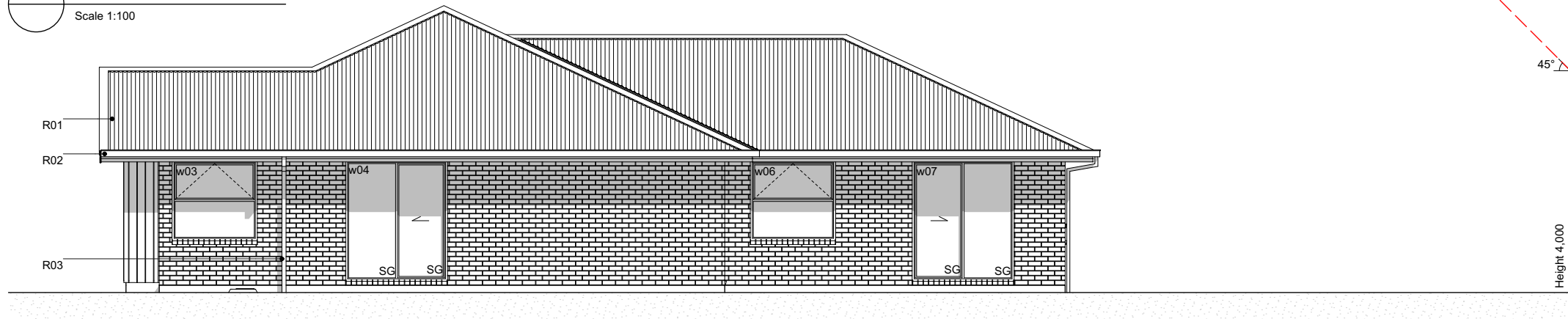
E-02 West Elevation Scale 1:100
