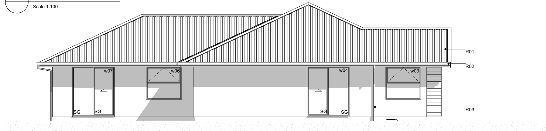
E-02 East Elevation Scale 1:100
