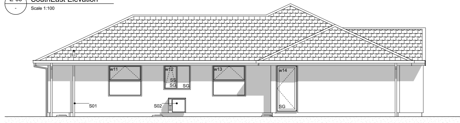
E-04 NorthEast Elevation Scale 1:100
