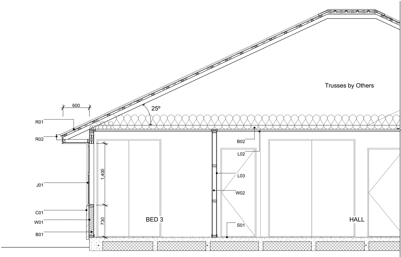
A Section A-A Scale 1:50
