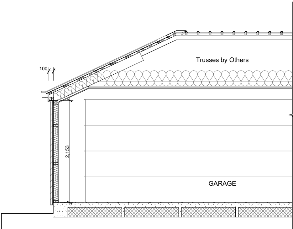
B Section B Scale 1:50
