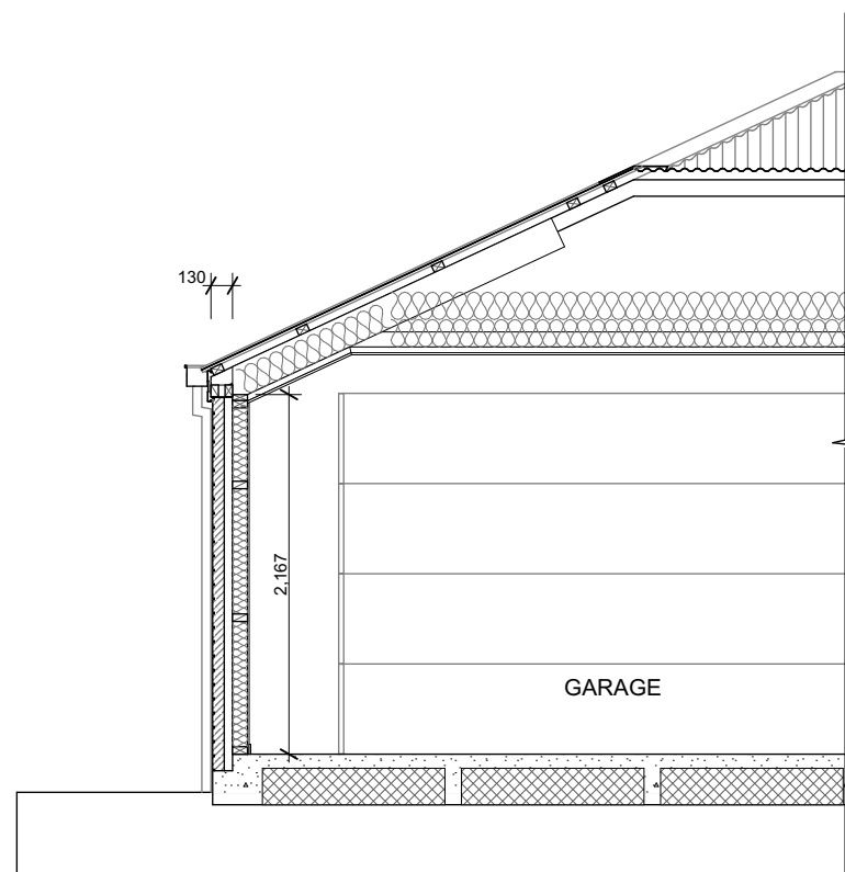
C Section C. Scale 1:50
