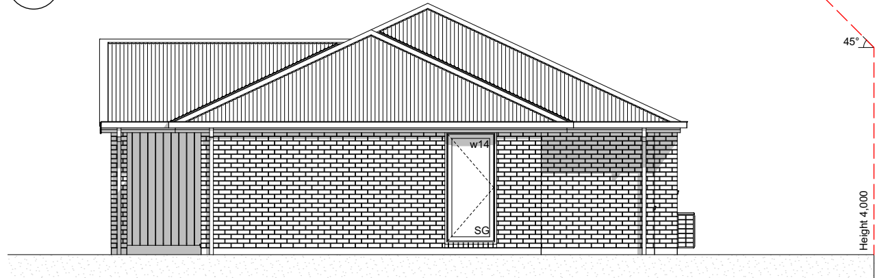
E-04 SouthEast Elevation Scale 1:100
