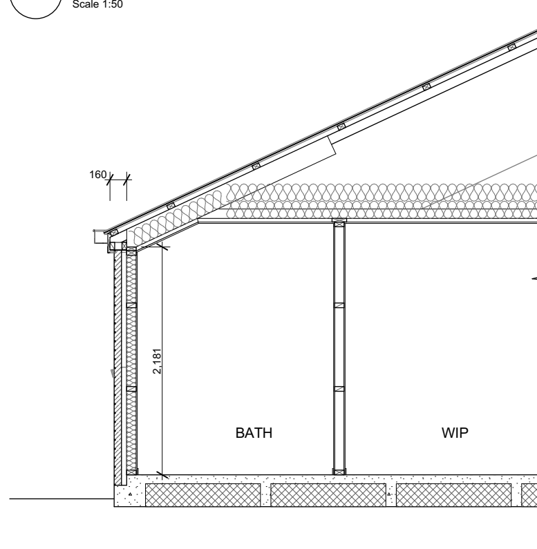
B Section B Scale 1:50
