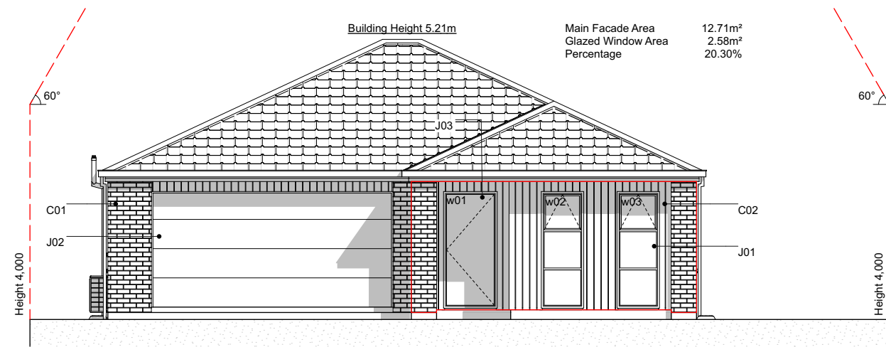
E-01 SouthEast Elevation Scale 1:100
