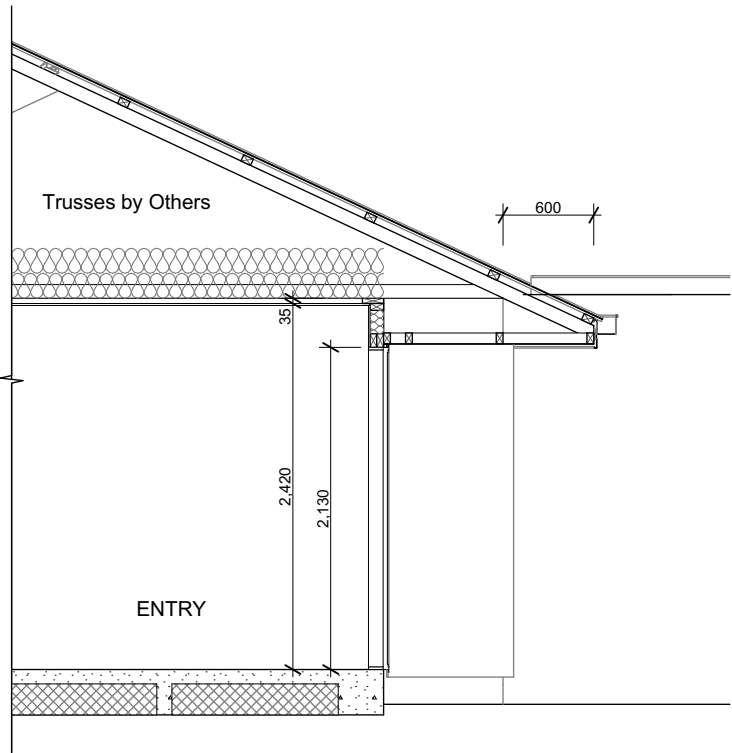
B Section B-B Scale 1:50
