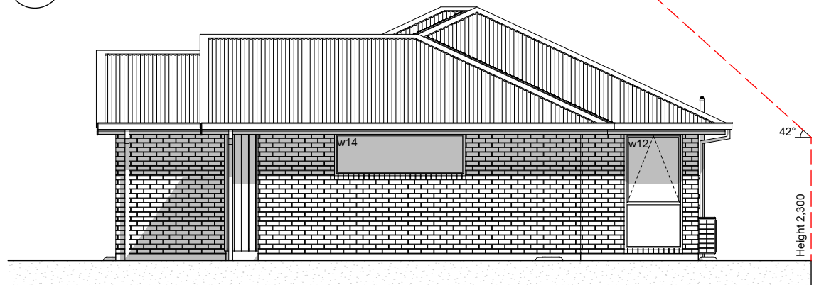
E-04 West Elevation Scale 1:100
