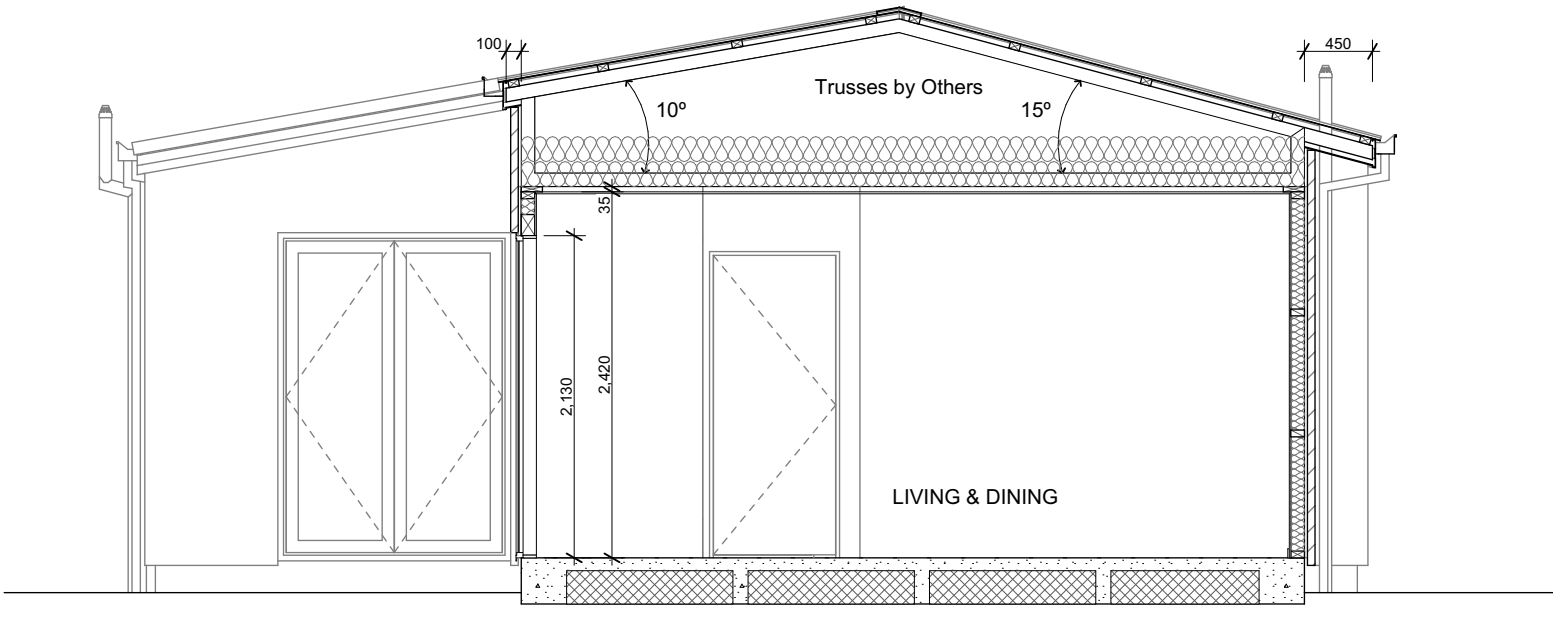
C Section C-C Scale 1:50
