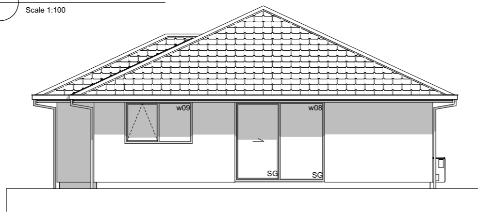
E-03 East Elevation Scale 1:100
