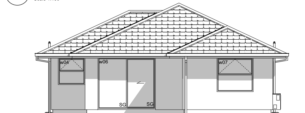
E-02 East Elevation Scale 1:100
