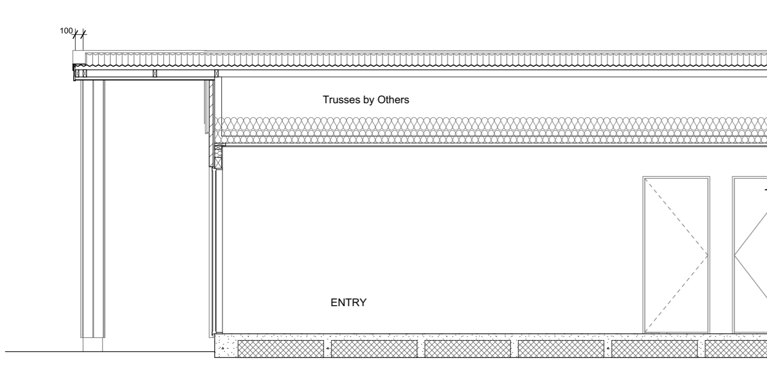
D Section D-D Scale 1:50
