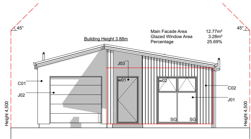
E-01 NorthEast Elevation Scale 1:100
