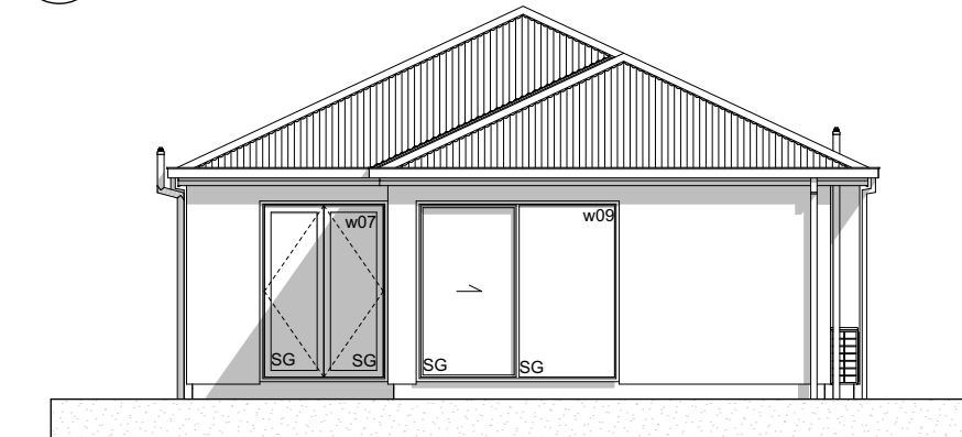
E-03 SouthWest Elevation Scale 1:100
