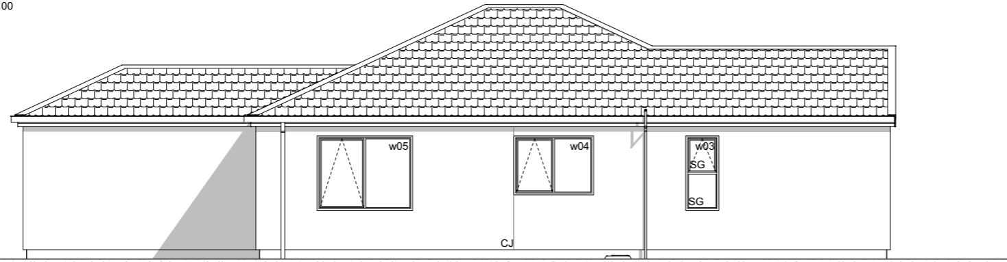
E-02 West Elevation Scale 1:100
