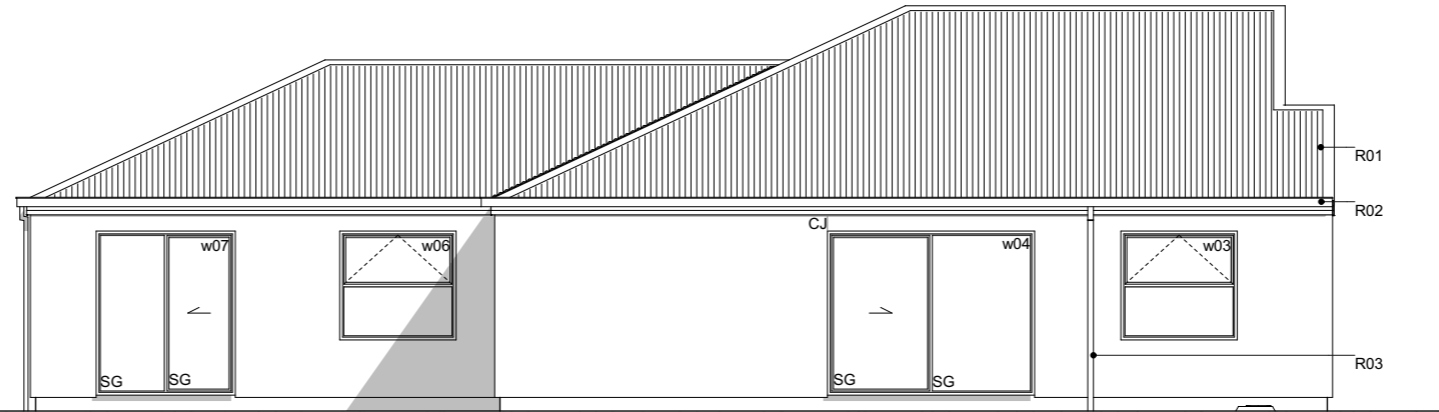
E-02 North Elevation
