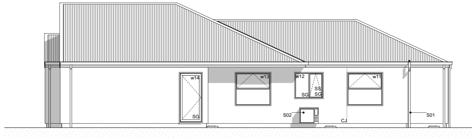
E-04 South Elevation
