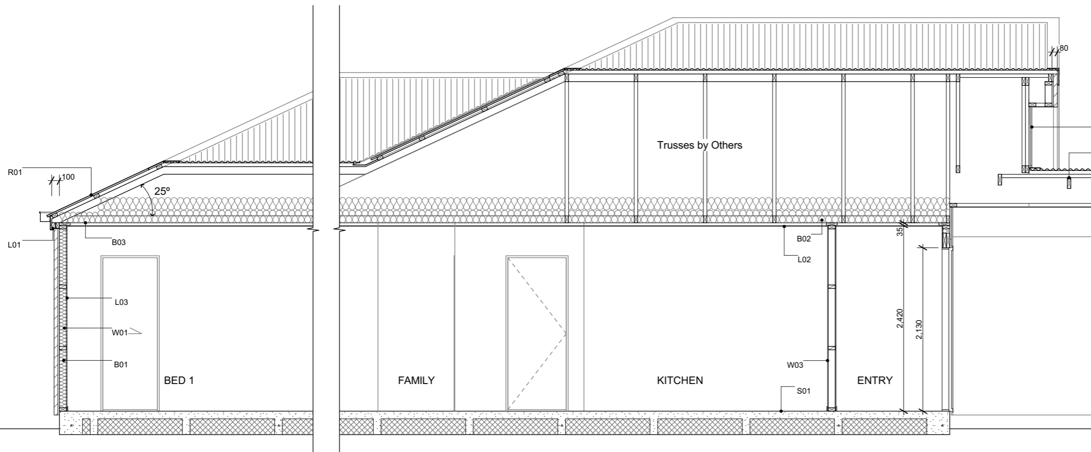
A Section A-A Scale 1:50
