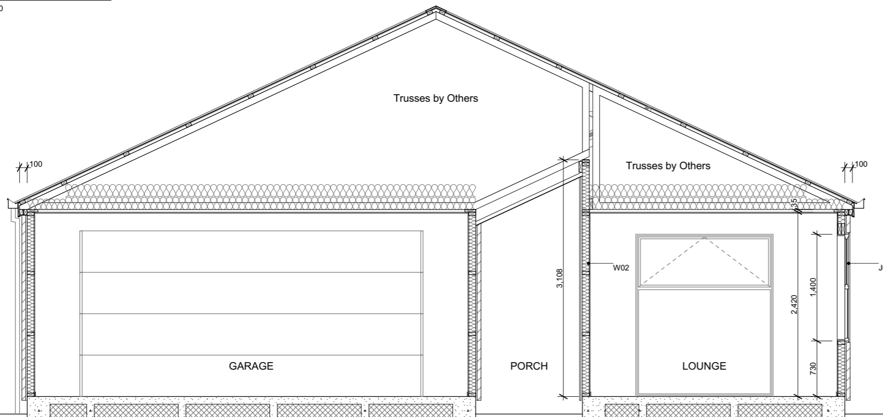
A Section A-A Scale 1:50
