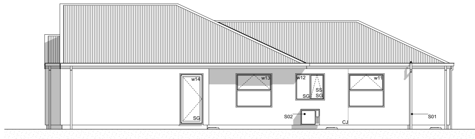
E-04 South Elevation Scale 1:100
