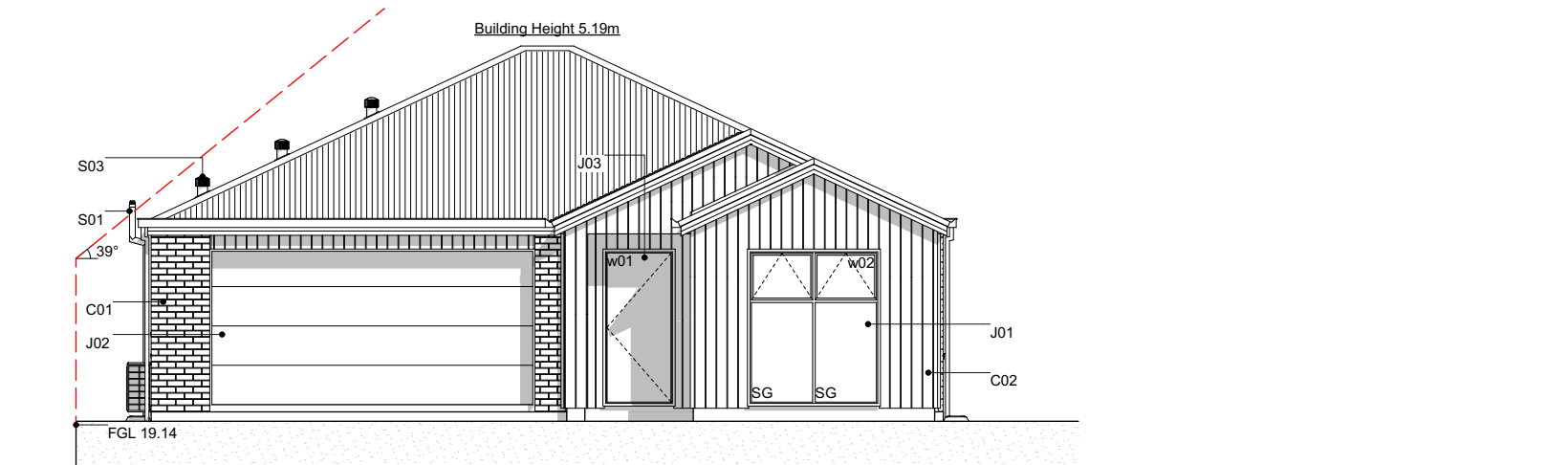
E-01 East Elevation Scale 1:100
