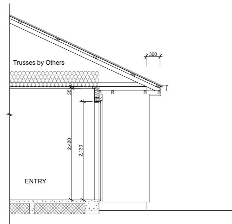
C Section C Scale 1:50
