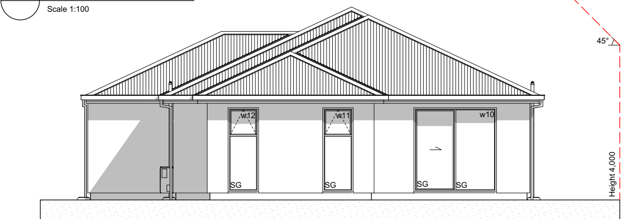
E-03 SouthWest Elevation Scale 1:100
