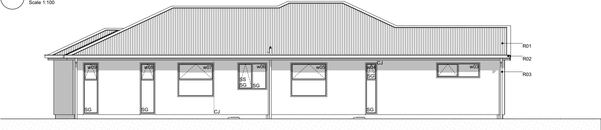
E-02 NorthWest Elevation Scale 1:100
