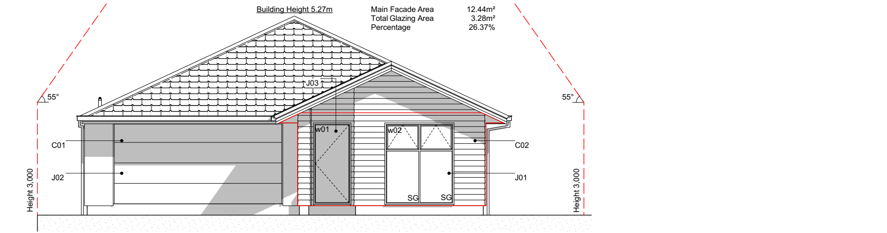
E-01 NorthEast Elevation #LayID Scale 1:100
