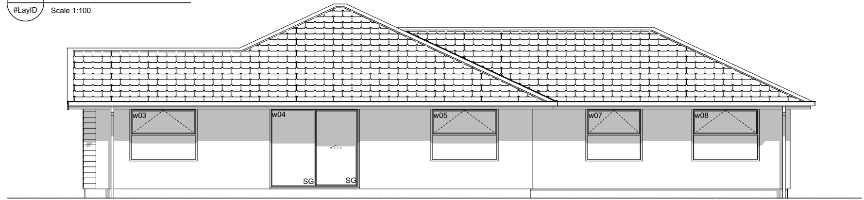
E-02 NorthWest Elevation #LayID Scale 1:100
