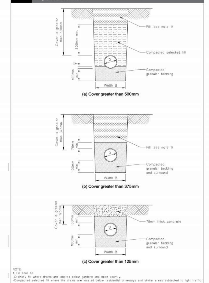
Figure 7 -G13/AS2 -Bedding and Backfilling
