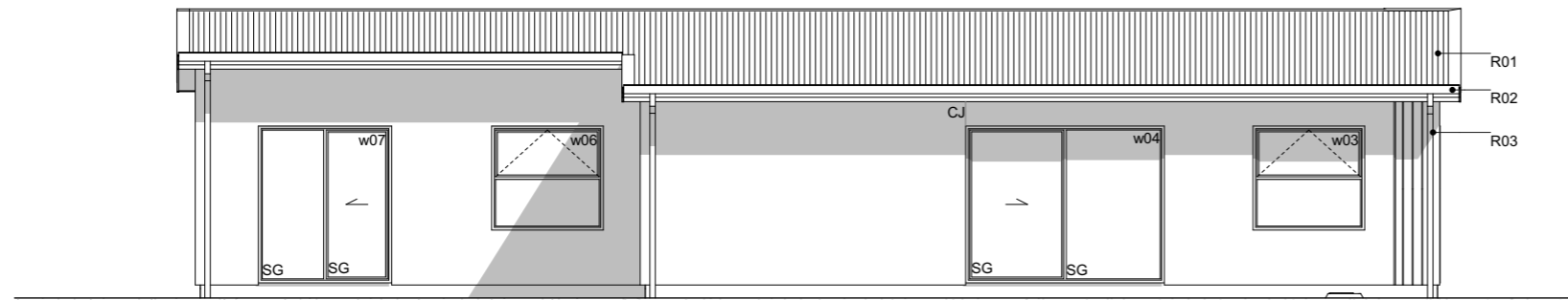
E-02 North Elevation Scale 1:100
