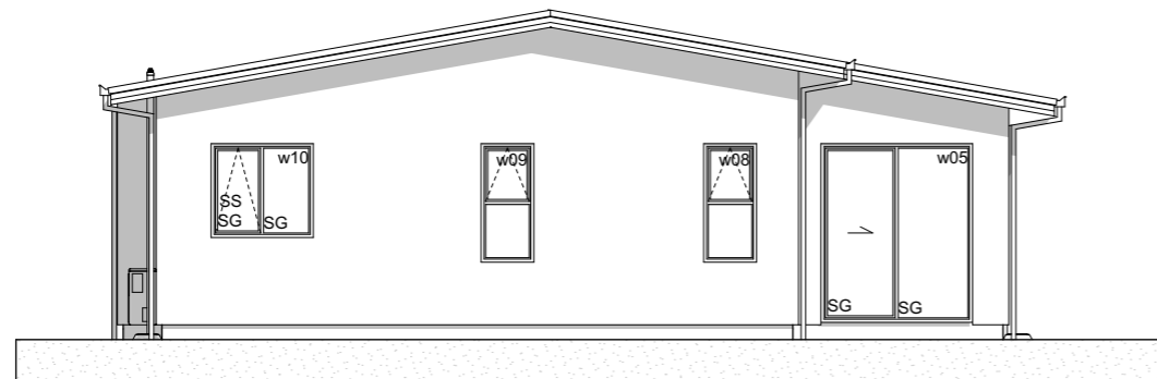
E-03 East Elevation Scale 1:100
