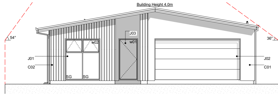
E-01 West Elevation Scale 1:100
