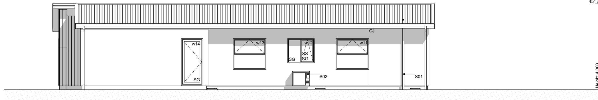
E-04 East Elevation Scale 1:100
