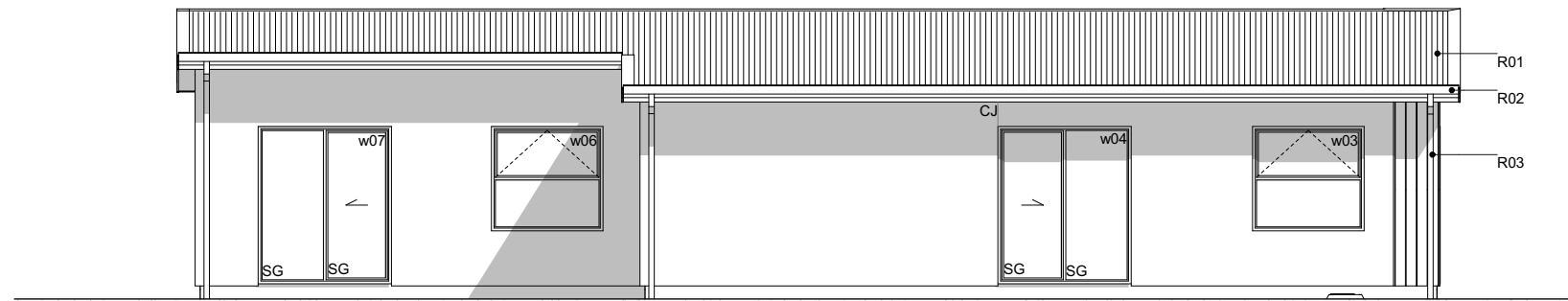
E-02 West Elevation Scale 1:100
