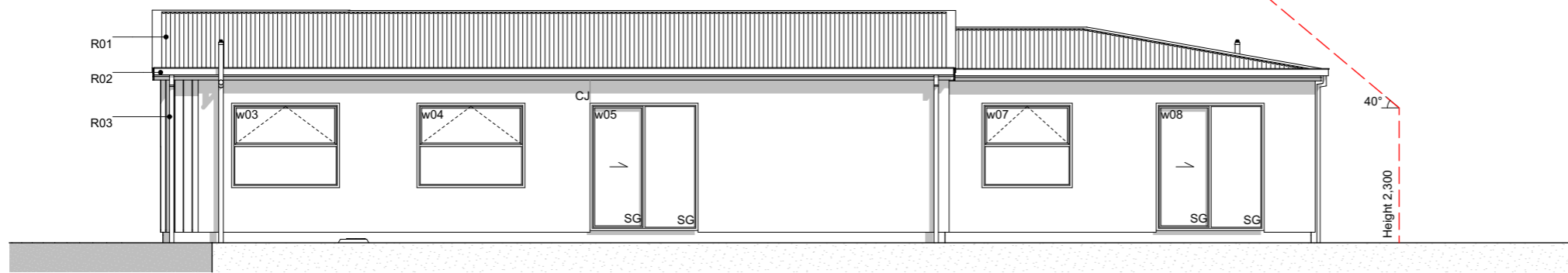
E-02 West Elevation Scale 1:100
