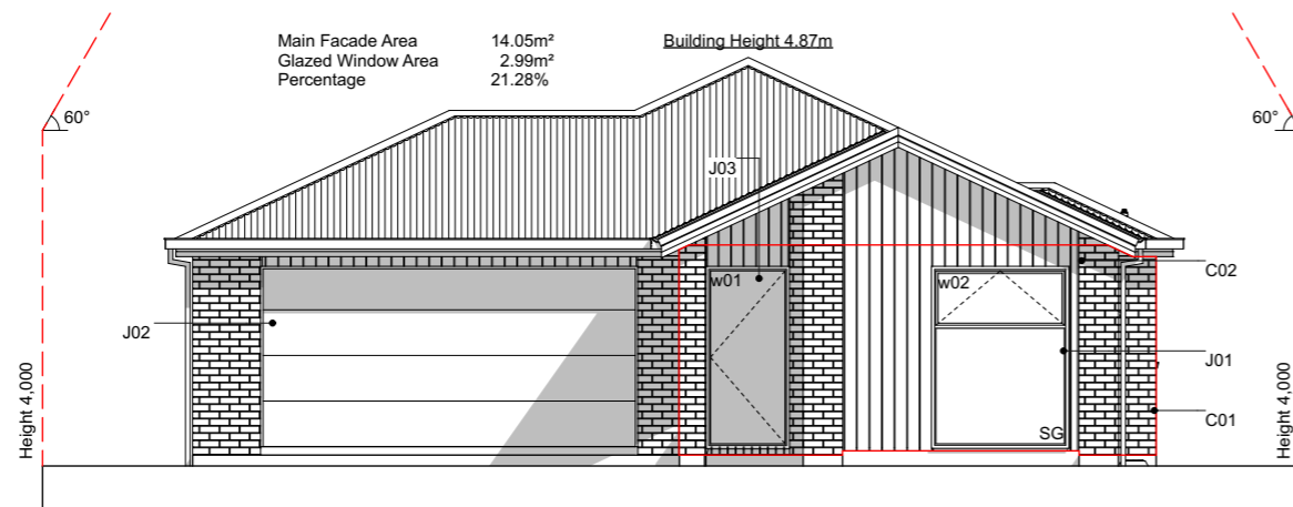
E-01 South Elevation Scale 1:100
