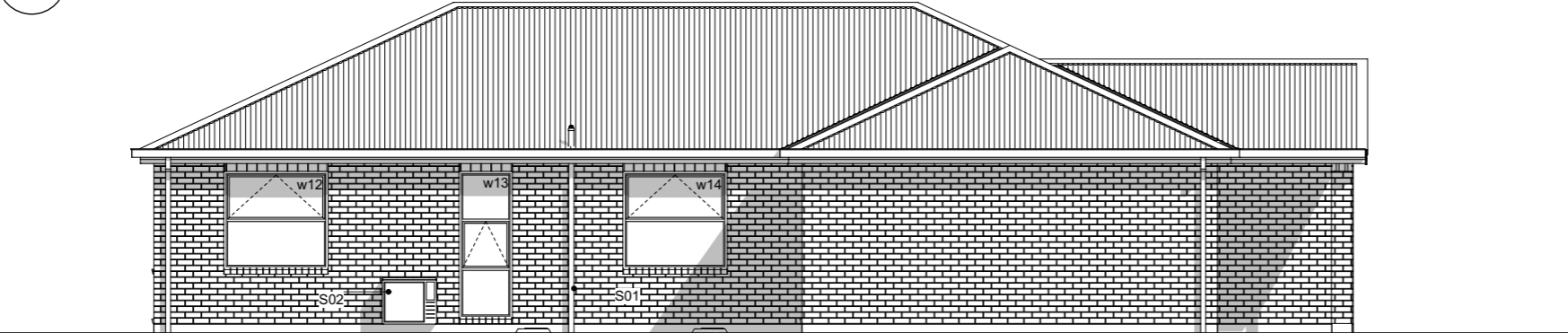
E-03 North Elevation Scale 1:100
