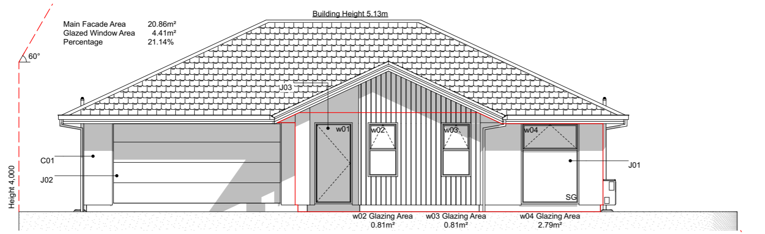
E-01 SouthWest Elevation Scale 1:100
