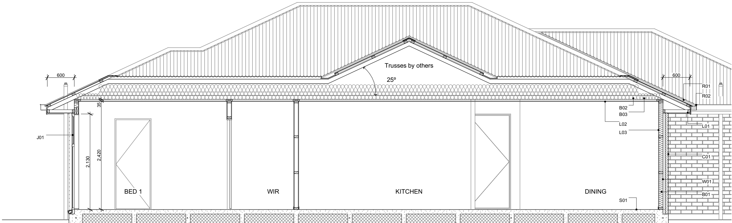
A Section A-A Scale 1:50
