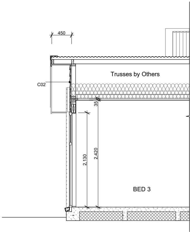
B Section B Scale 1:50
