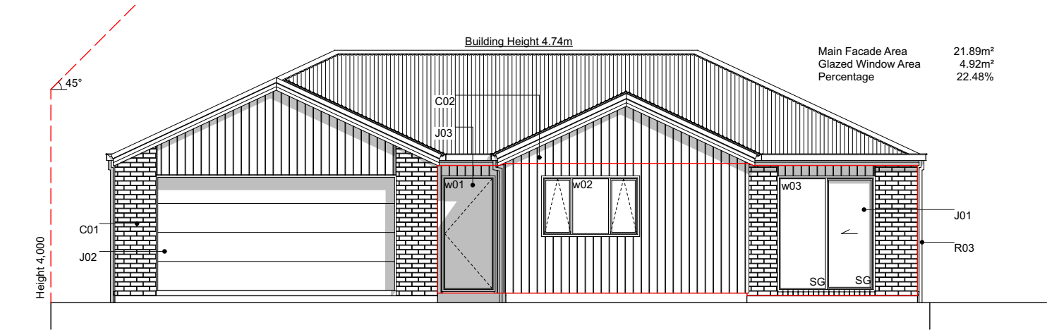
E-01 East Elevation Scale 1:100
