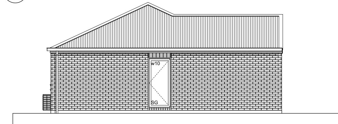
E-04 South Elevation Scale 1:100
