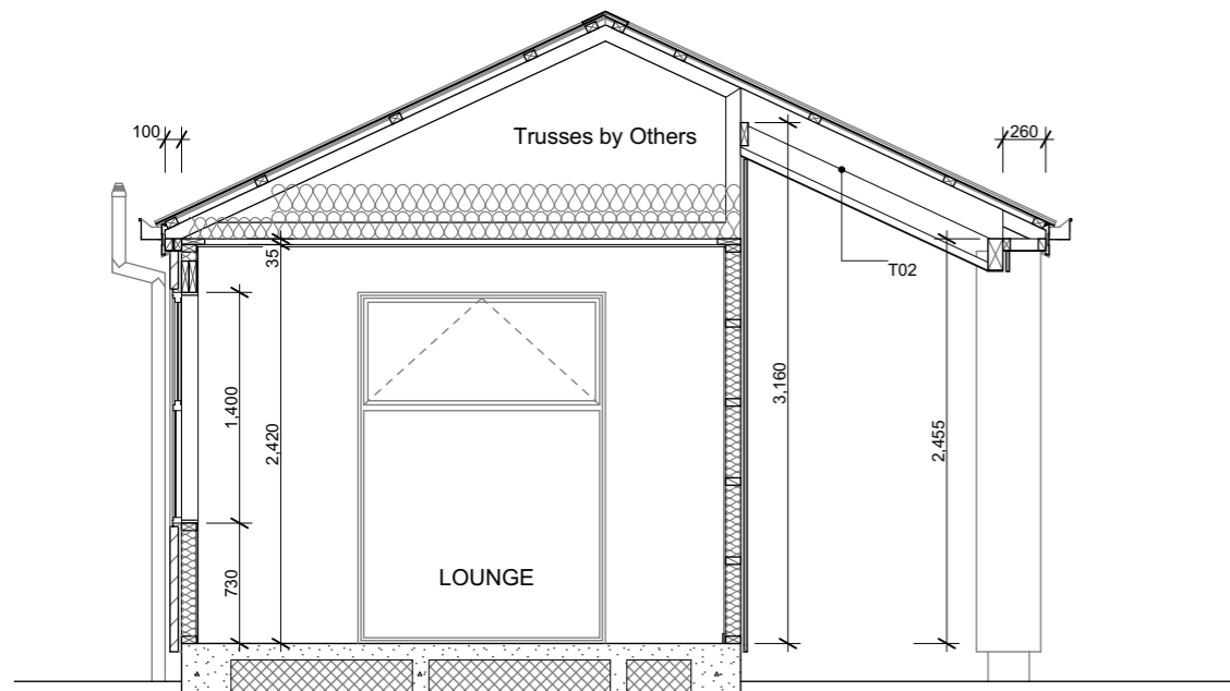
B Section B Scale 1:50
