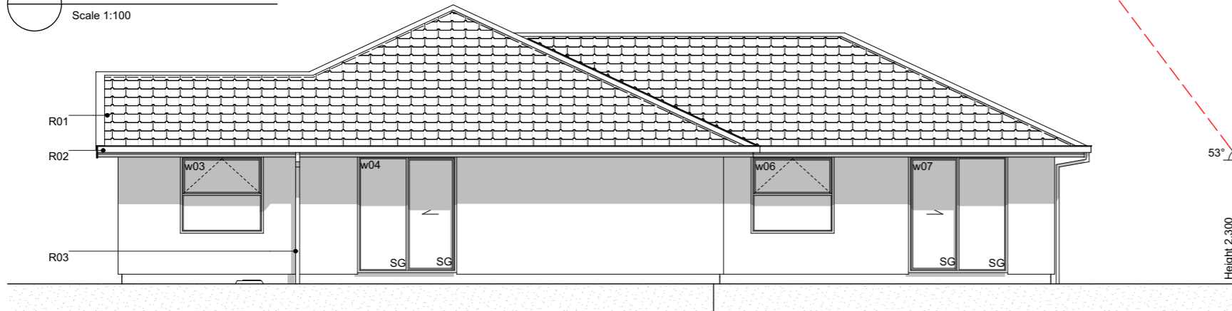
E-02 NorthEast Elevation Scale 1:100
