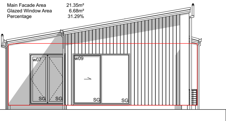
E-03 NorthWest Elevation Scale 1:100
