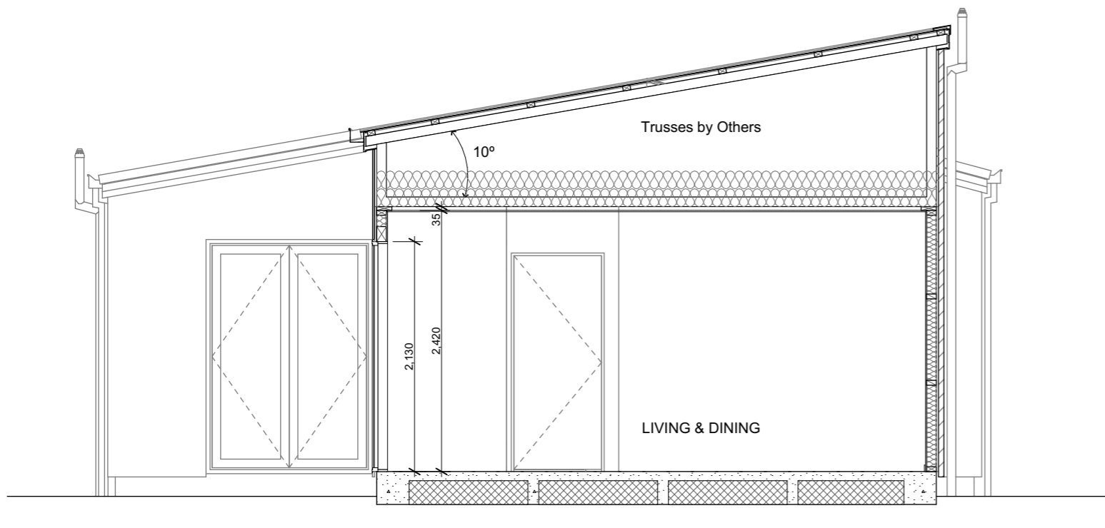
C Section C-C Scale 1:50
