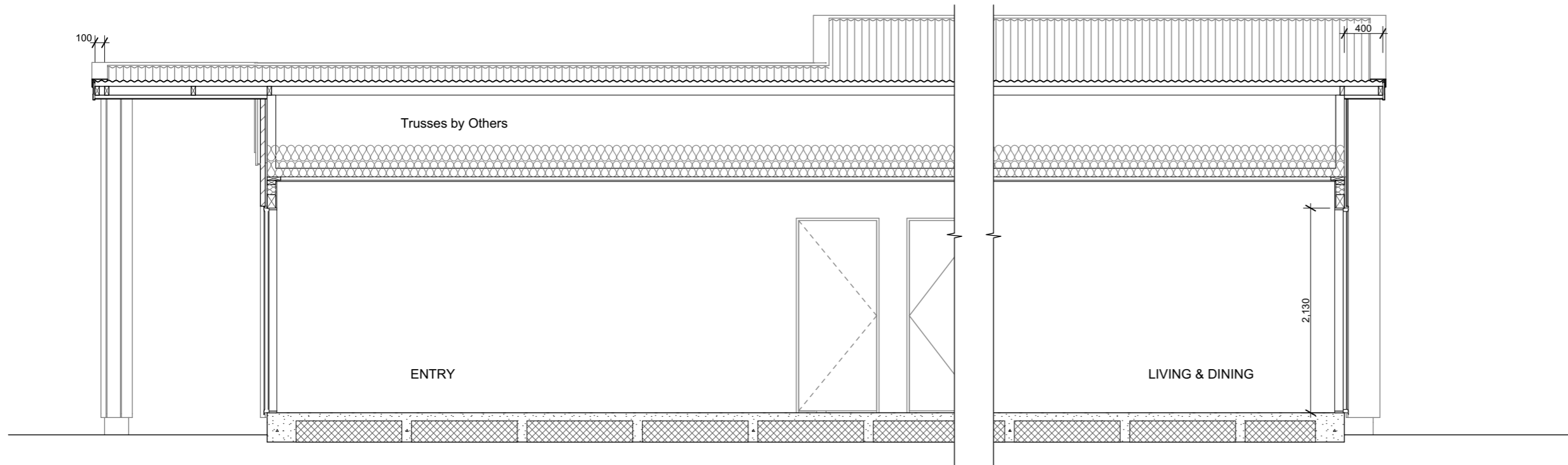
D Section D-D Scale 1:50
