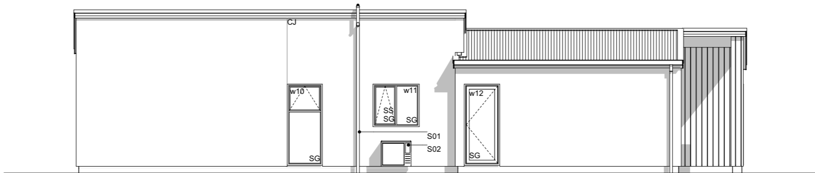
E-03 NorthWest Elevation Scale 1:100
