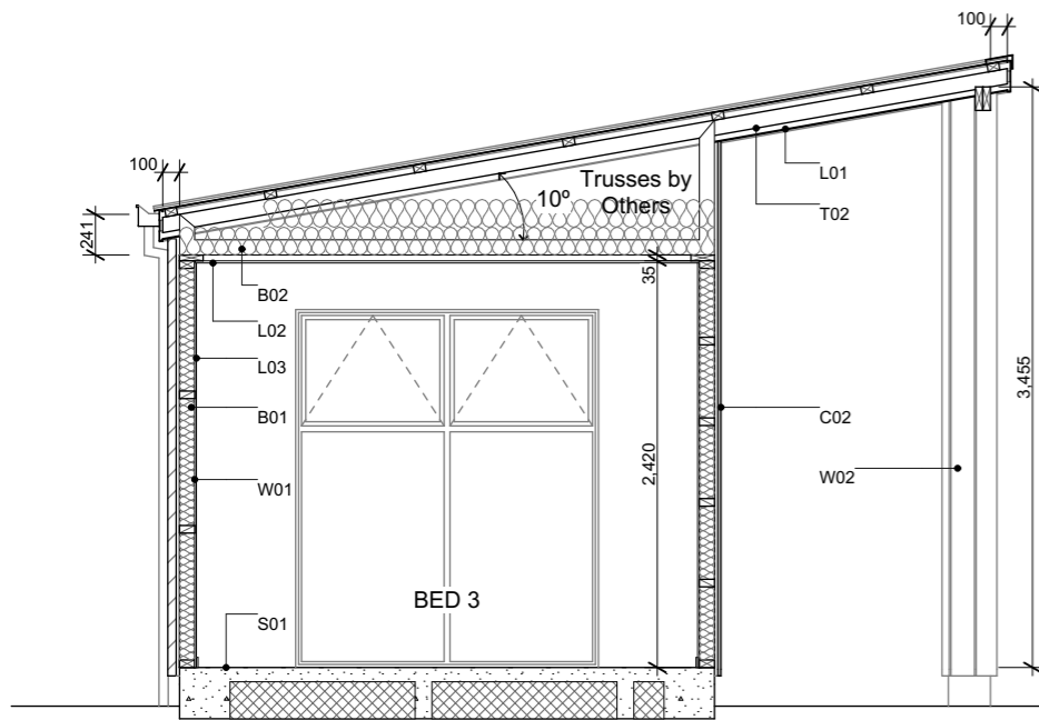
A Section A-A Scale 1:50
