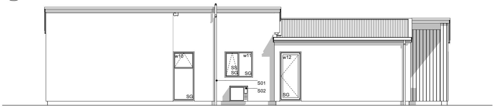
E-03 NorthWest Elevation Scale 1:100
