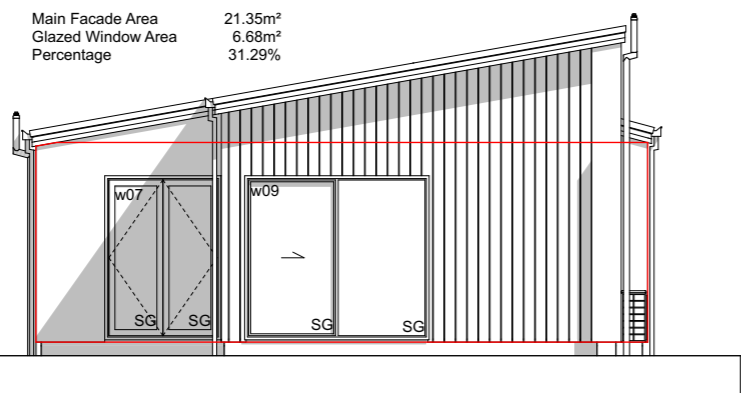
E-03 NorthWest Elevation Scale 1:100
