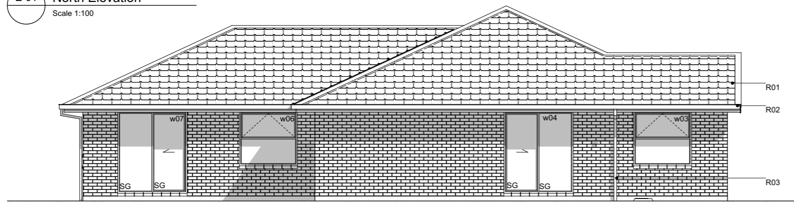
E-02 East Elevation Scale 1:100
