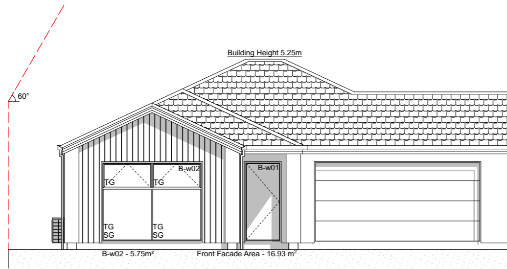
E-01 SouthEast Elevation Scale 1:100
