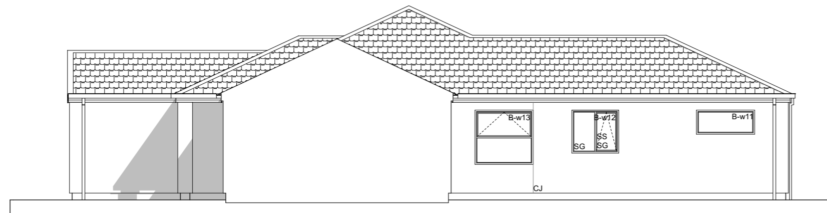
E-06 NorthEast (Lot 81) Elevation Scale 1:100
