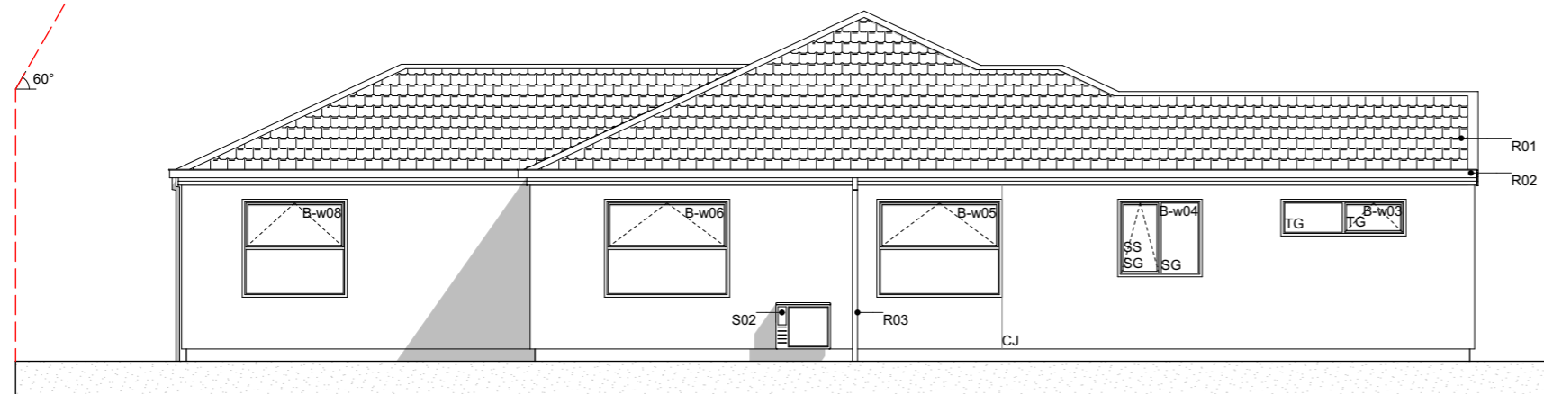
E-05 SouthWest (Lot 81) Elevation Scale 1:100
