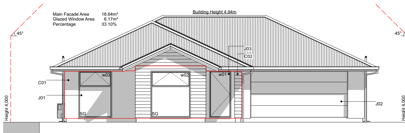
E-01 SouthWest Elevation Scale 1:100
