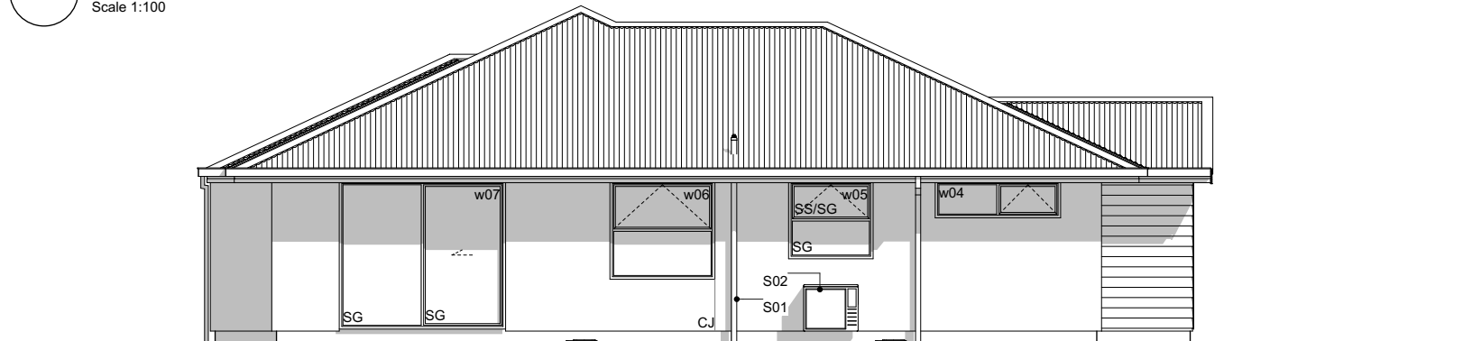
E-02 NorthWest Elevation Scale 1:100
