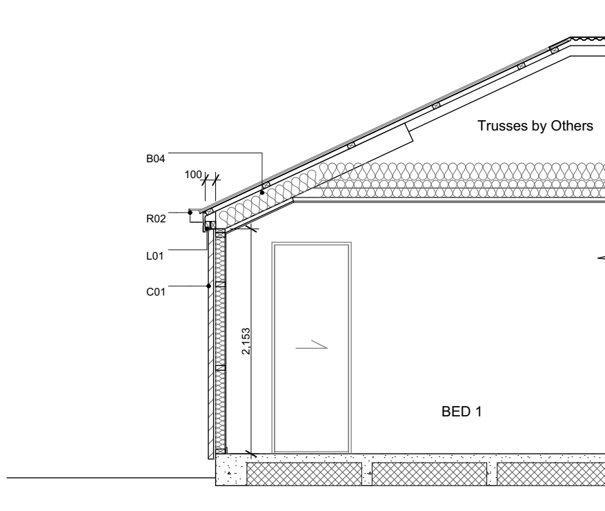
B Section B Scale 1:50
