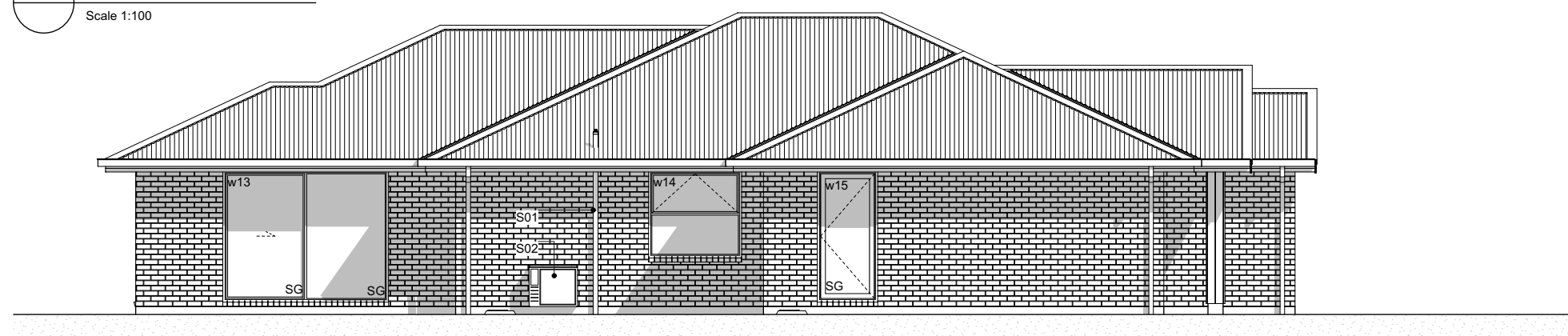
E-04 West Elevation Scale 1:100
