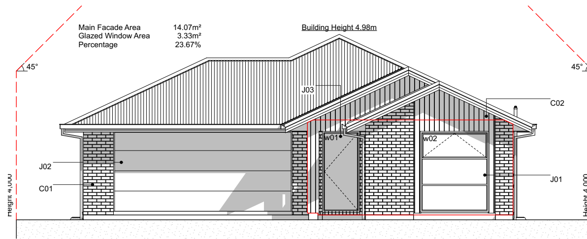
E-01 South Elevation Scale 1:100
