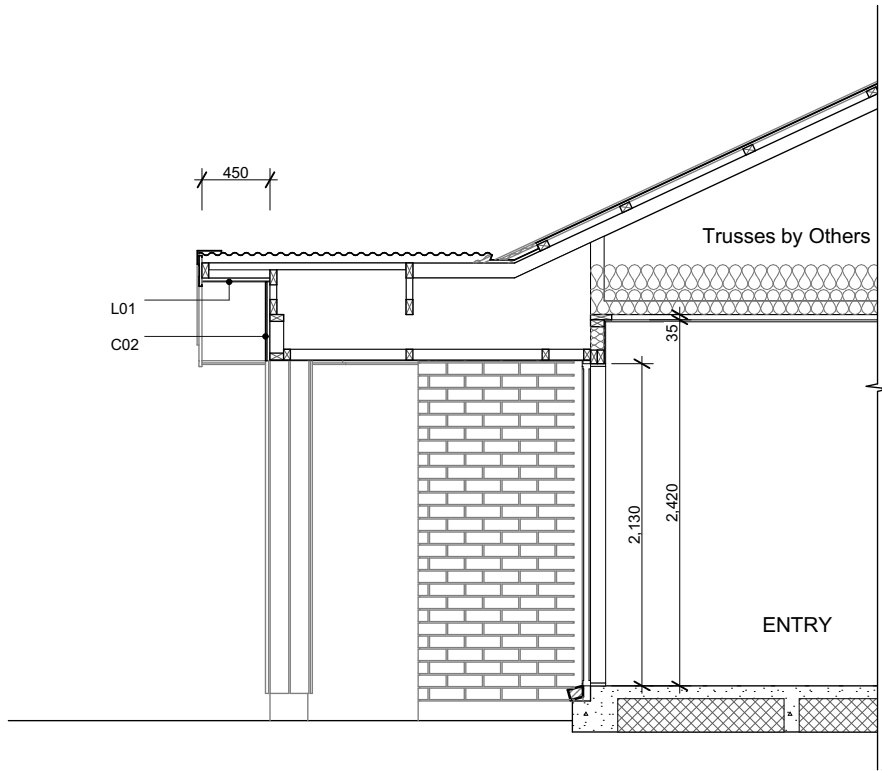
B Section B #LayID Scale 1:50
