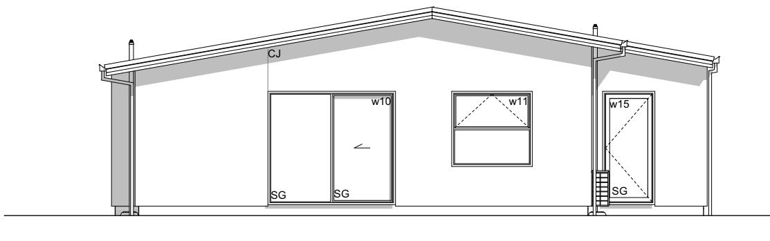
E-03 North Elevation Scale 1:100
