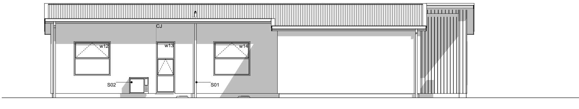
E-04 West Elevation Scale 1:100
