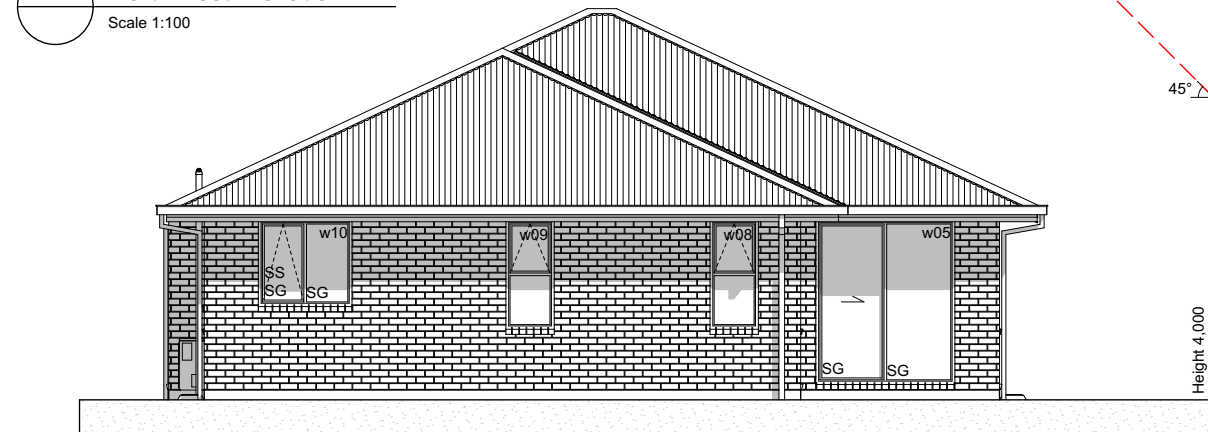
E-03 NorthEast Elevation Scale 1:100
