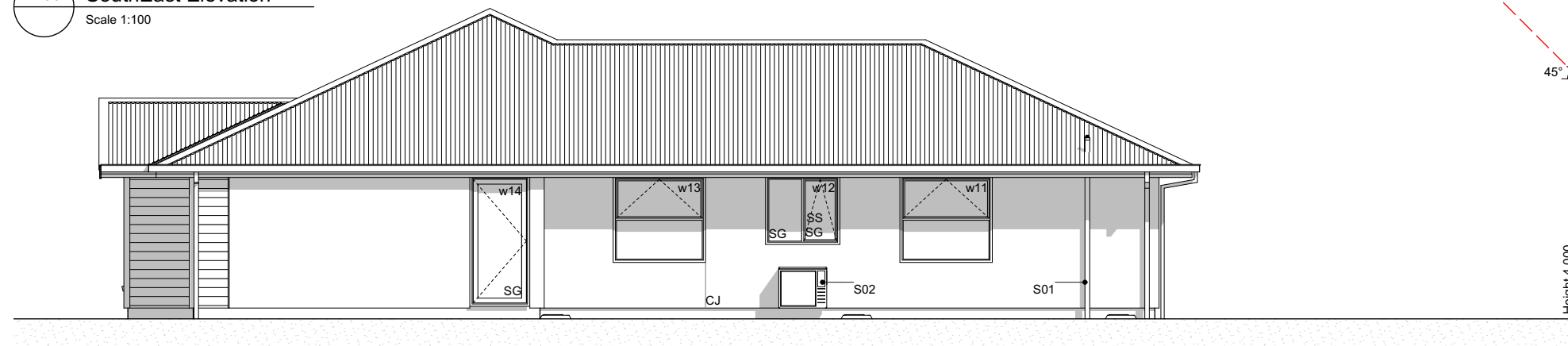
E-04 SouthEast Elevation Scale 1:100
