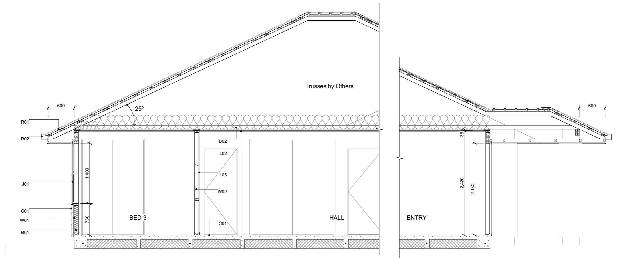
A Section A-A #LayID Scale 1:50
