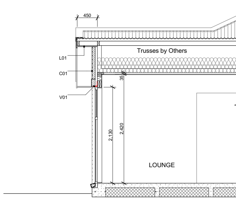
B Section B Scale 1:50
