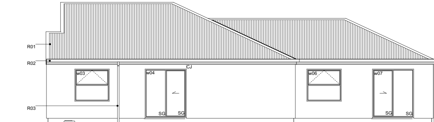
E-02 NorthWest Elevation Scale 1:100
