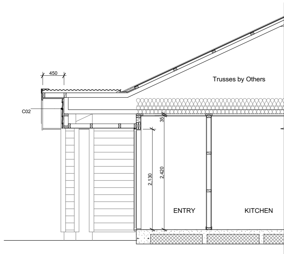
B Section B Scale 1:50
